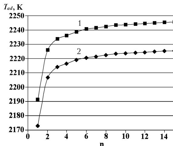
Fig. 1. Theoretical combustion temperature T_T = T_{ad} of air mixtures of n-alkanes C_nH_{2n+2} (in dependence of number of carbon atoms): 1 – dry air; 2 – wet air, H_2O vapour content d = 24.4 g H_2O /kg dry air. Fuel-oxidant mixture temperature 300 K, air excess factor \lambda = 1.05 .
